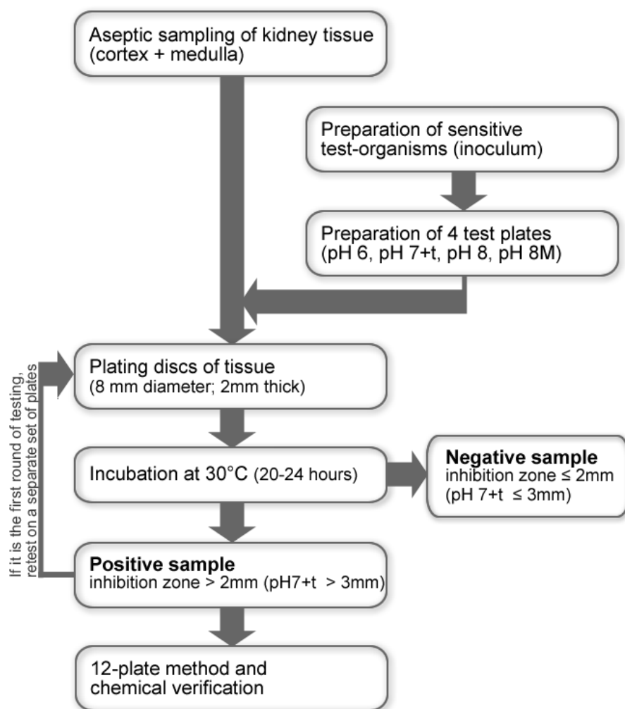
Fig. 2. Schematic representation of the 4-plate method (adapted from Birgitte Herbert Nielsen).
