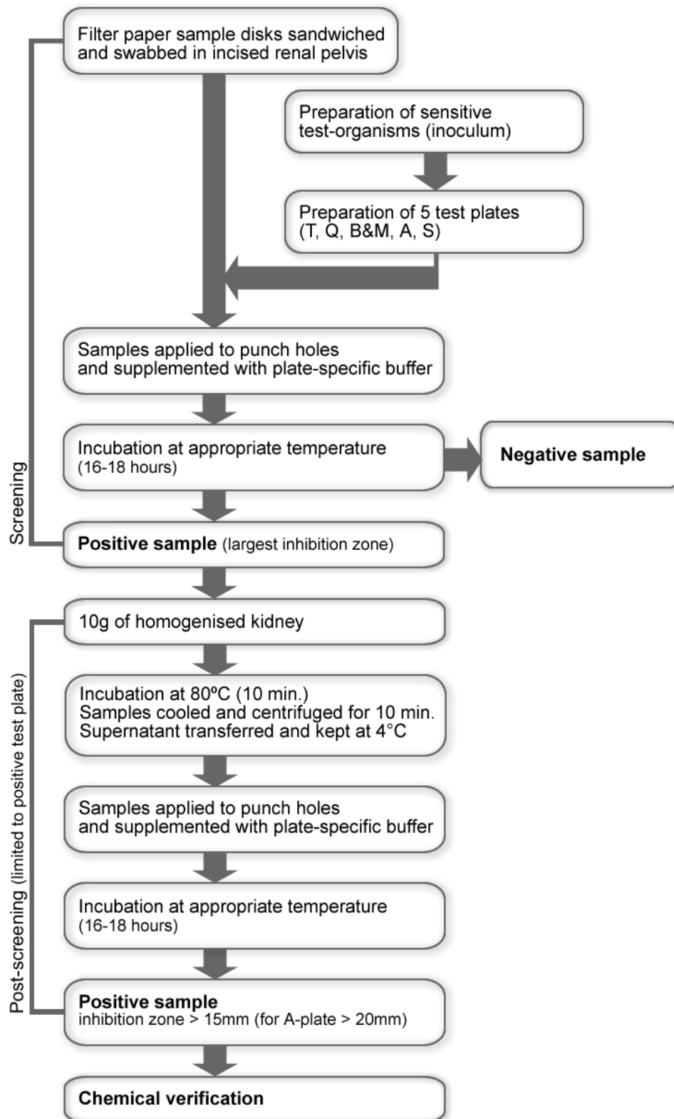
Fig. 3. Schematic representation of the Nouws antibiotic test (adapted from Mariel Pikkemaat).
